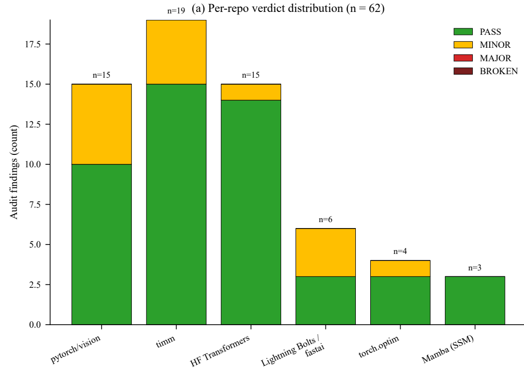
Figure 4 — Audit calibration at n = 62 (third-party trusted repos)
