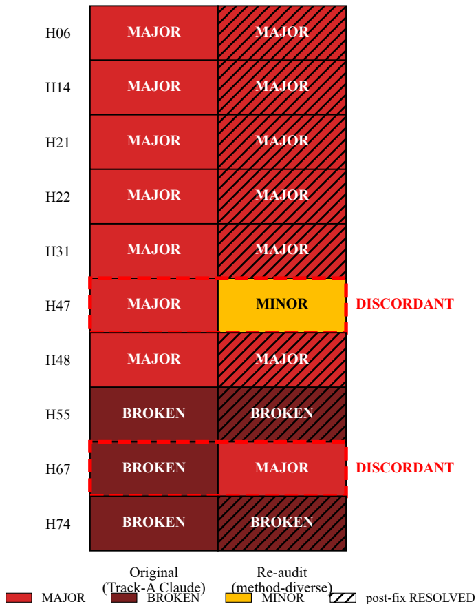
Figure 5 — Cross-family re-audit concordance (8/10 CONCORDANT, 2/10 DISCORDANT)
