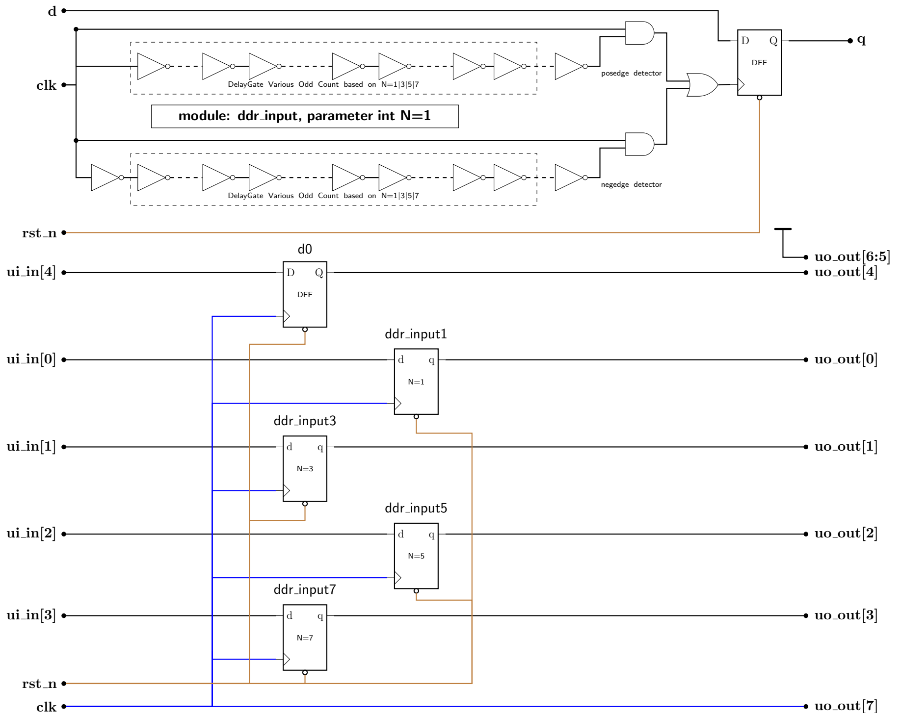
Double Data Rate Throughput Test
