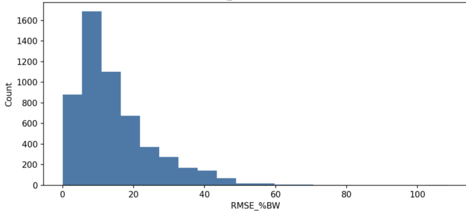
RMSE_%BW histogram
