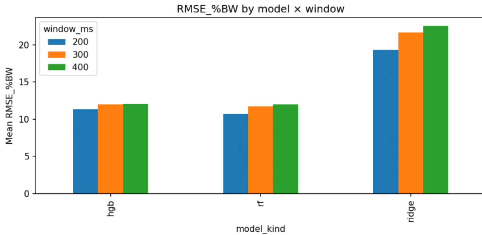
RMSE by model × window
