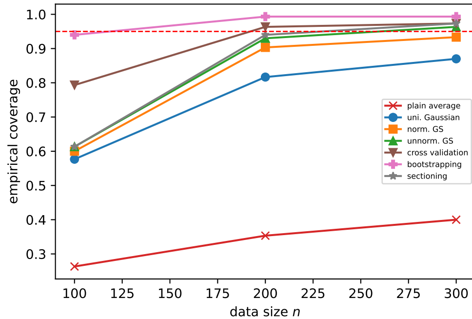
paper_saa (split=0.7)
