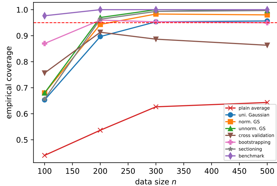
paper_so (split=0.7)
