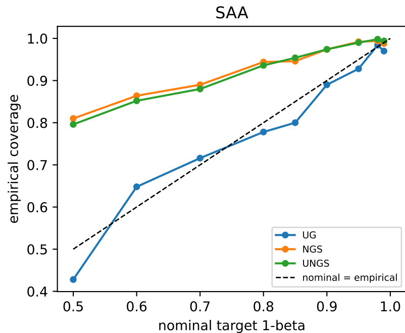
Calibration: empirical coverage vs nominal 1-beta (points on/above dashed = valid/conservative)
