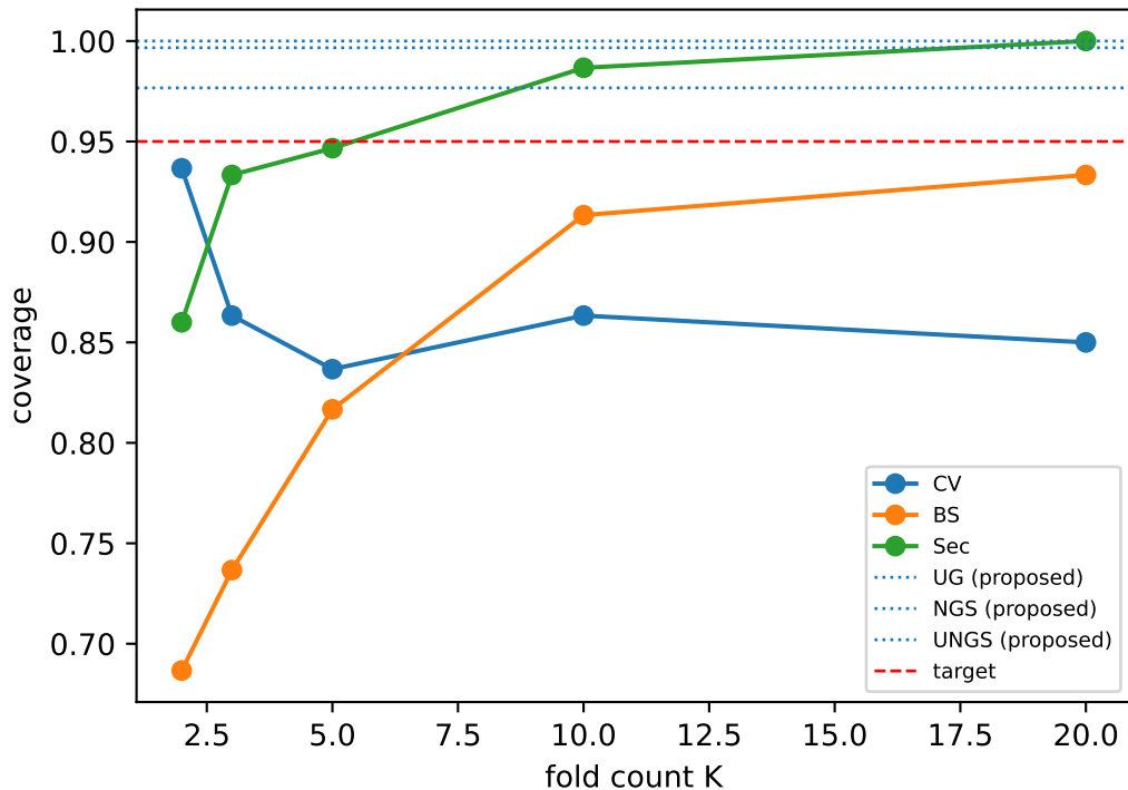
SO N=1000: coverage vs fold count K
