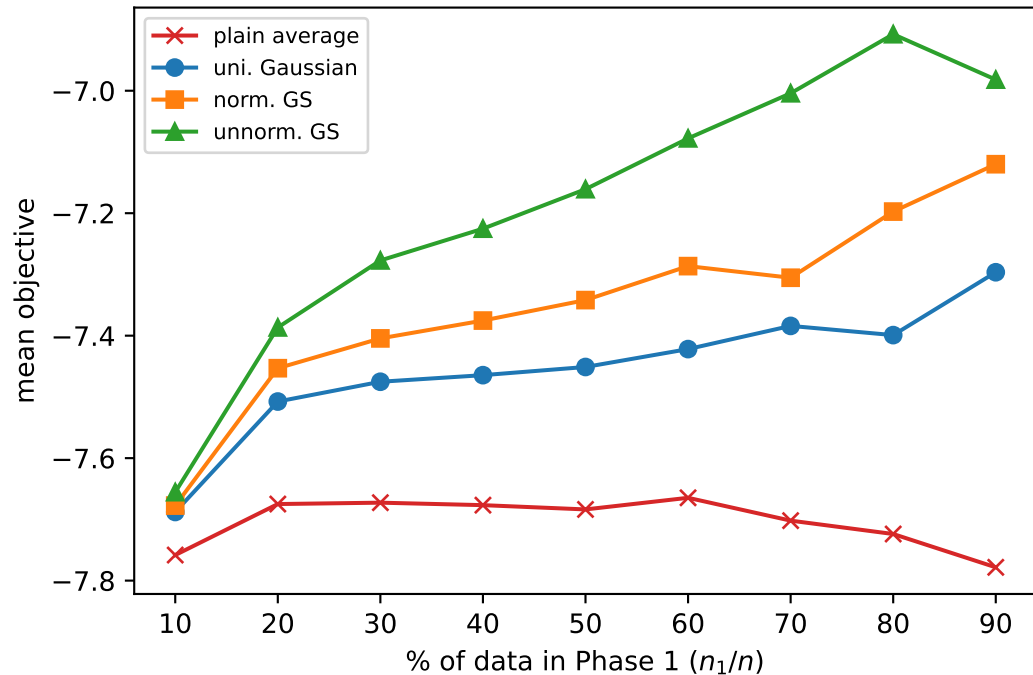
SO: objective vs Phase-1 fraction
