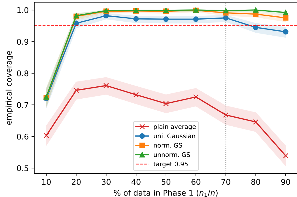
SO: coverage vs Phase-1 fraction
