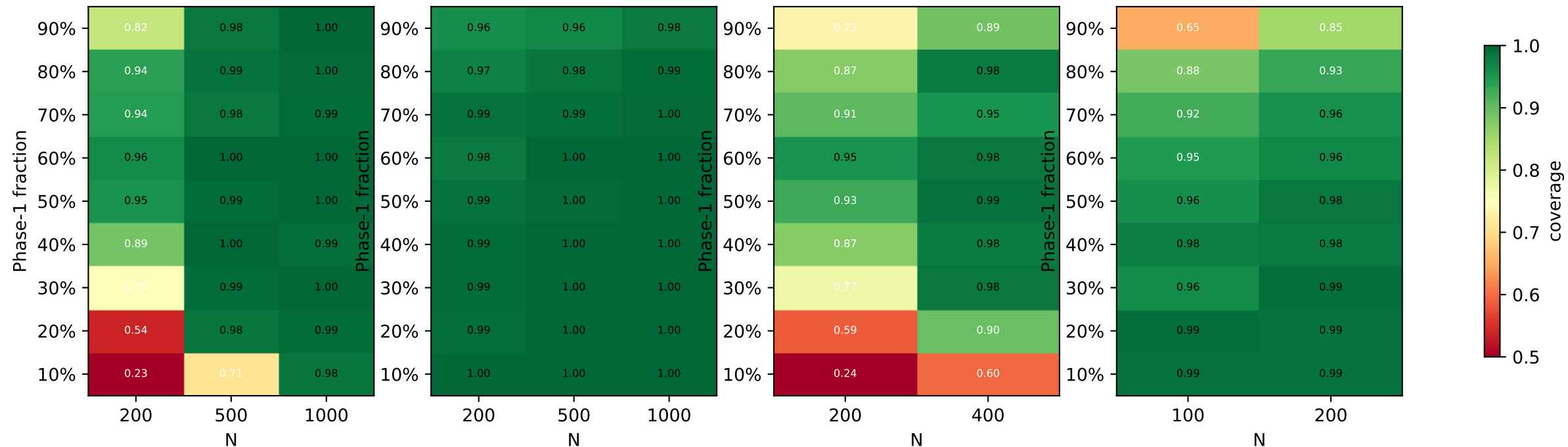
Coverage over (Phase-1 fraction x N) at d=10 (NGS) (green \geq 0.95 target)
