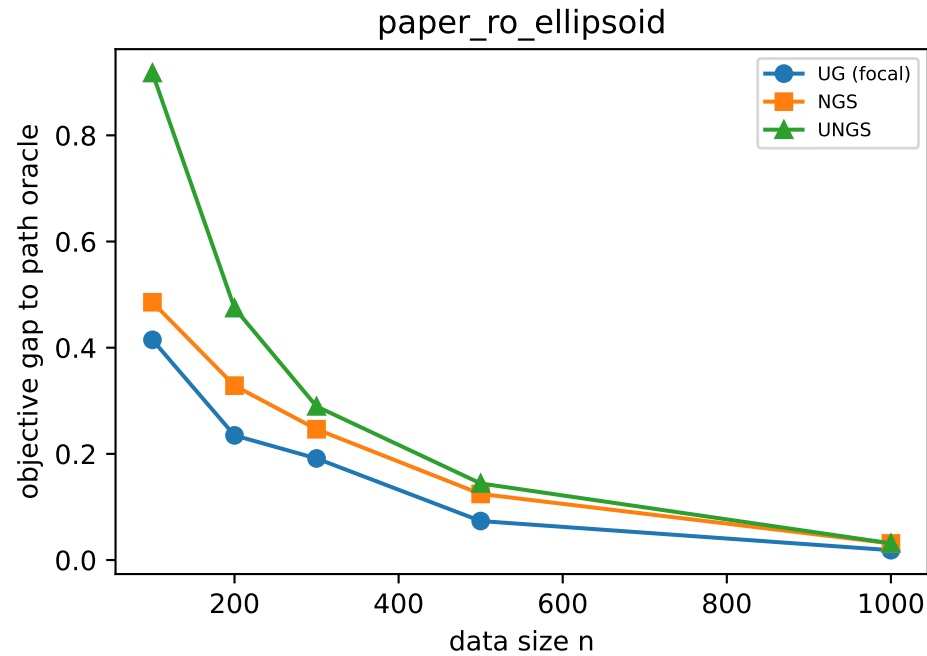
Objective gap to oracle shrinks with n
