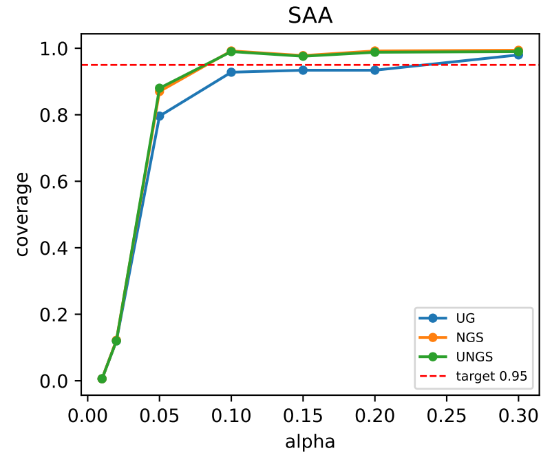
Coverage vs tolerance parameter alpha (target 0.95)
