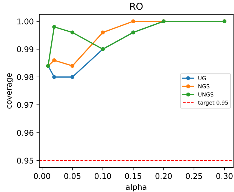
Coverage vs tolerance parameter alpha (target 0.95)
