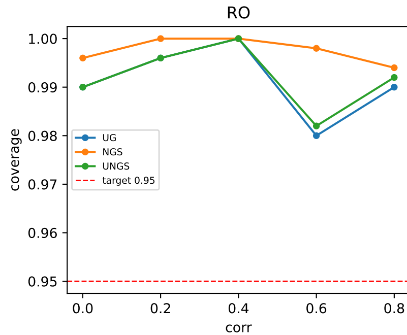
Coverage vs correlation, d=10 (target 0.95)
