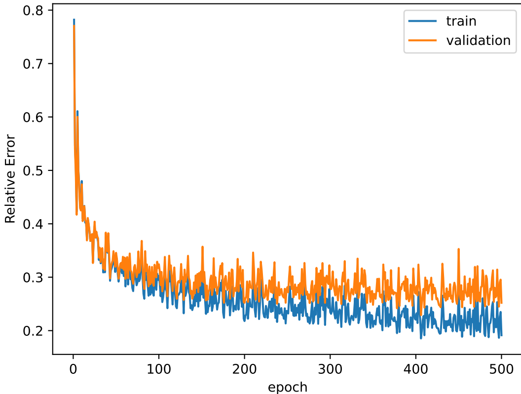
Sphere: Relative Error: Relative Error
