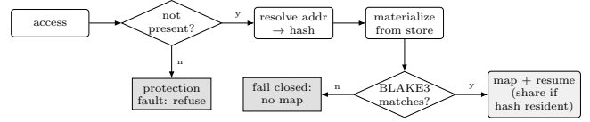
Figure 2: The residency and fault path (F1, F2, F3). A miss is a verified materialize-by-hash. A protection fault and a verification failure are each refused at the fault boundary, and an already-resident hash is shared.
