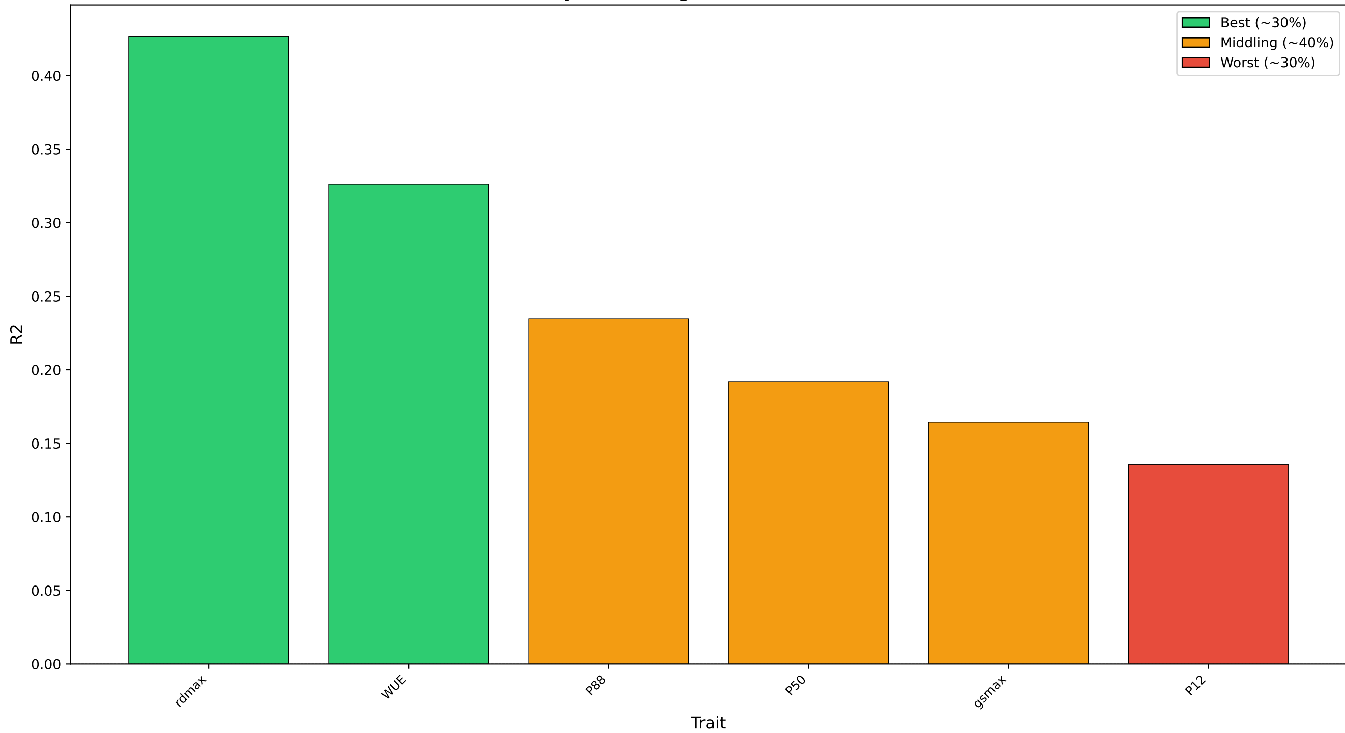
R 2 by Trait (Original Scale - Pooled)
