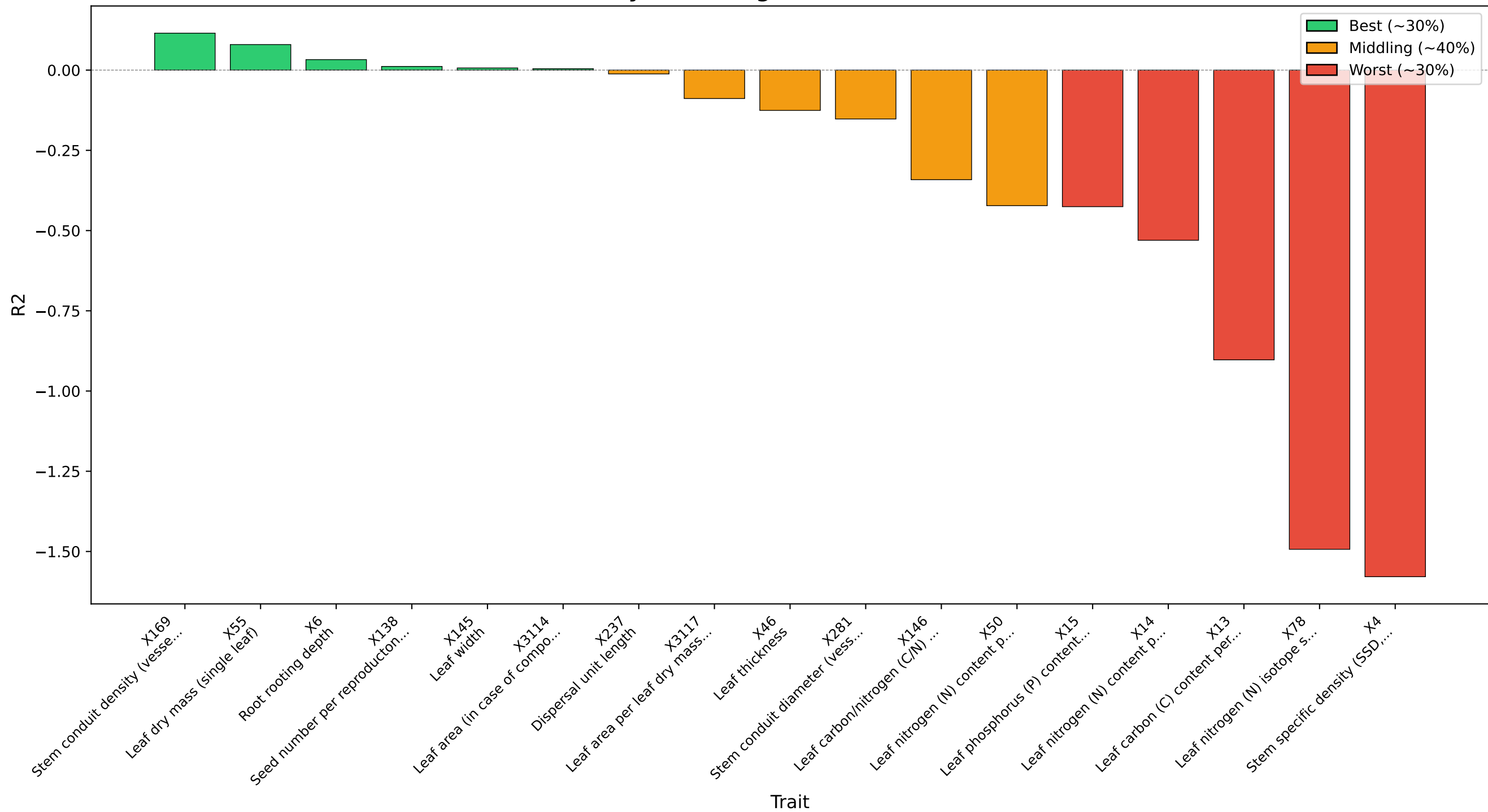
R 2 by Trait (Original Scale - Pooled)
