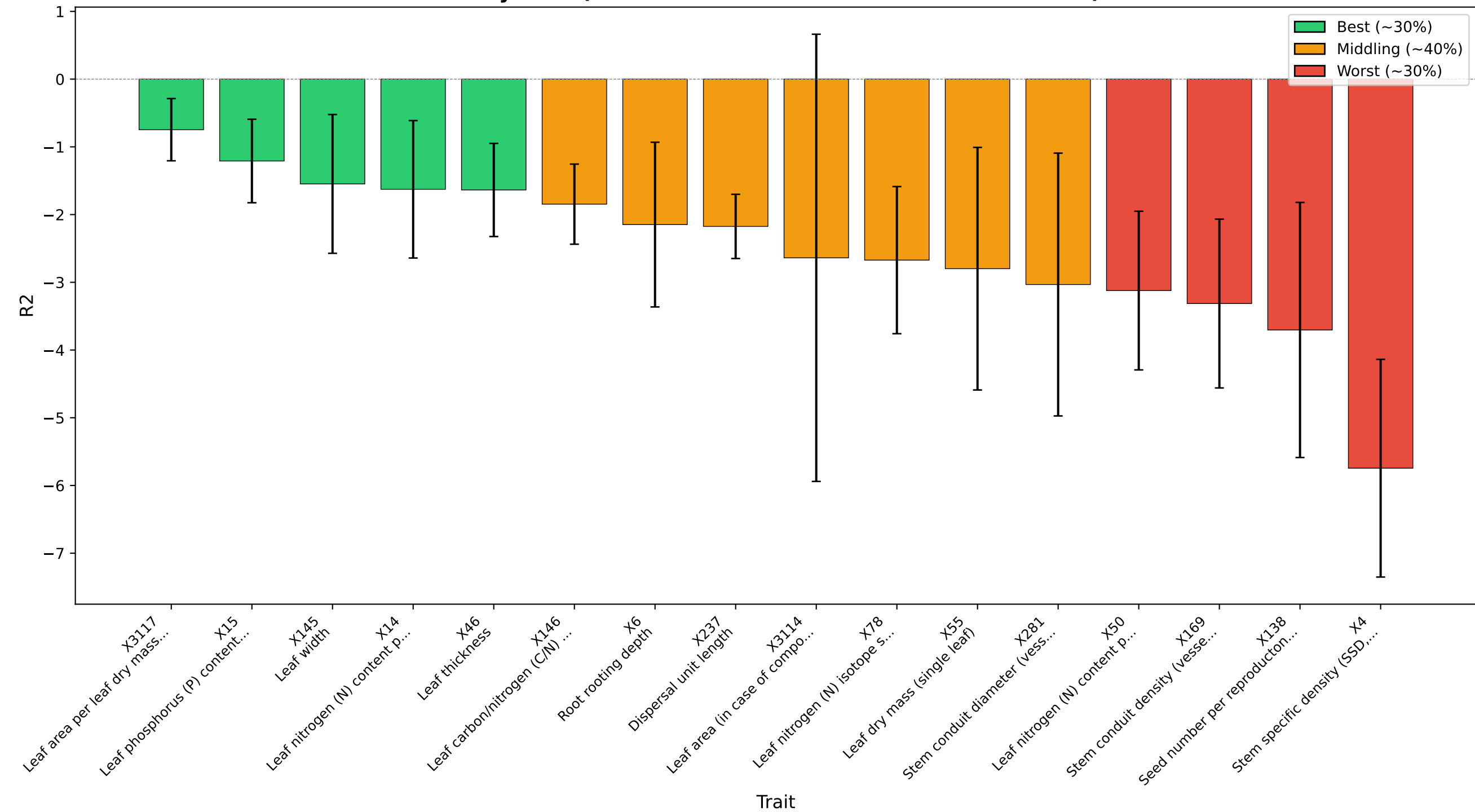
R 2 by Trait (Transformed Scale - Fold-wise Mean \pm Std)
