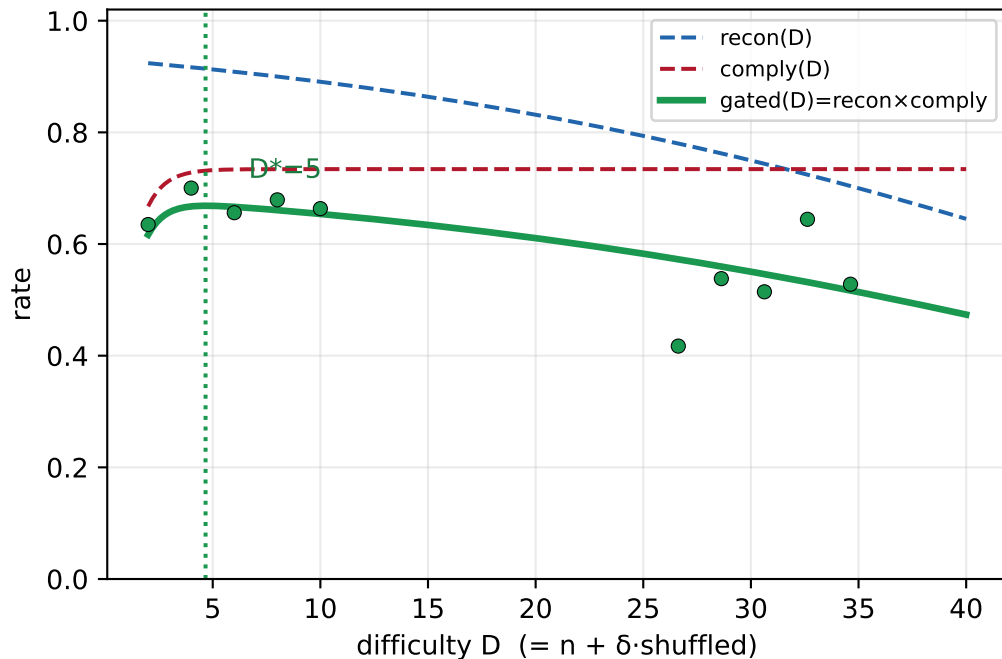
Qwen2.5-7B (weaker reconstructor)
