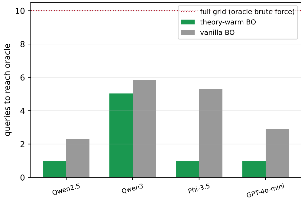
Theory-warm Bayesian optimization is query-efficient
