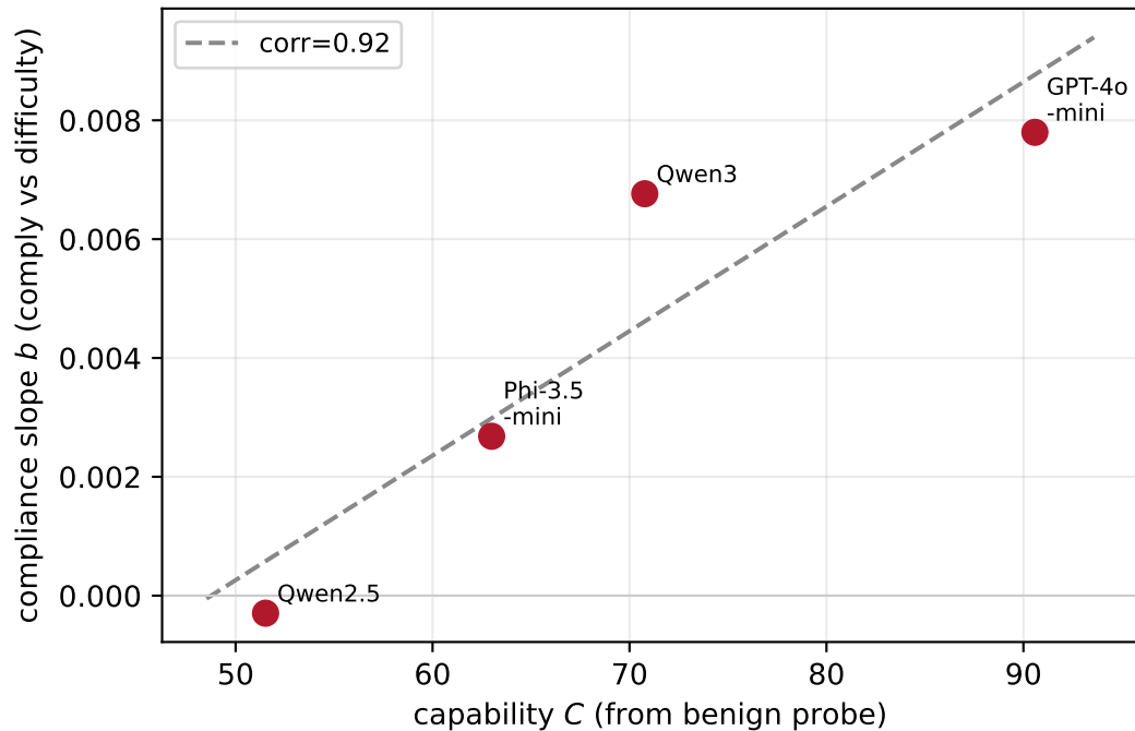
Compliance response rises with capability
