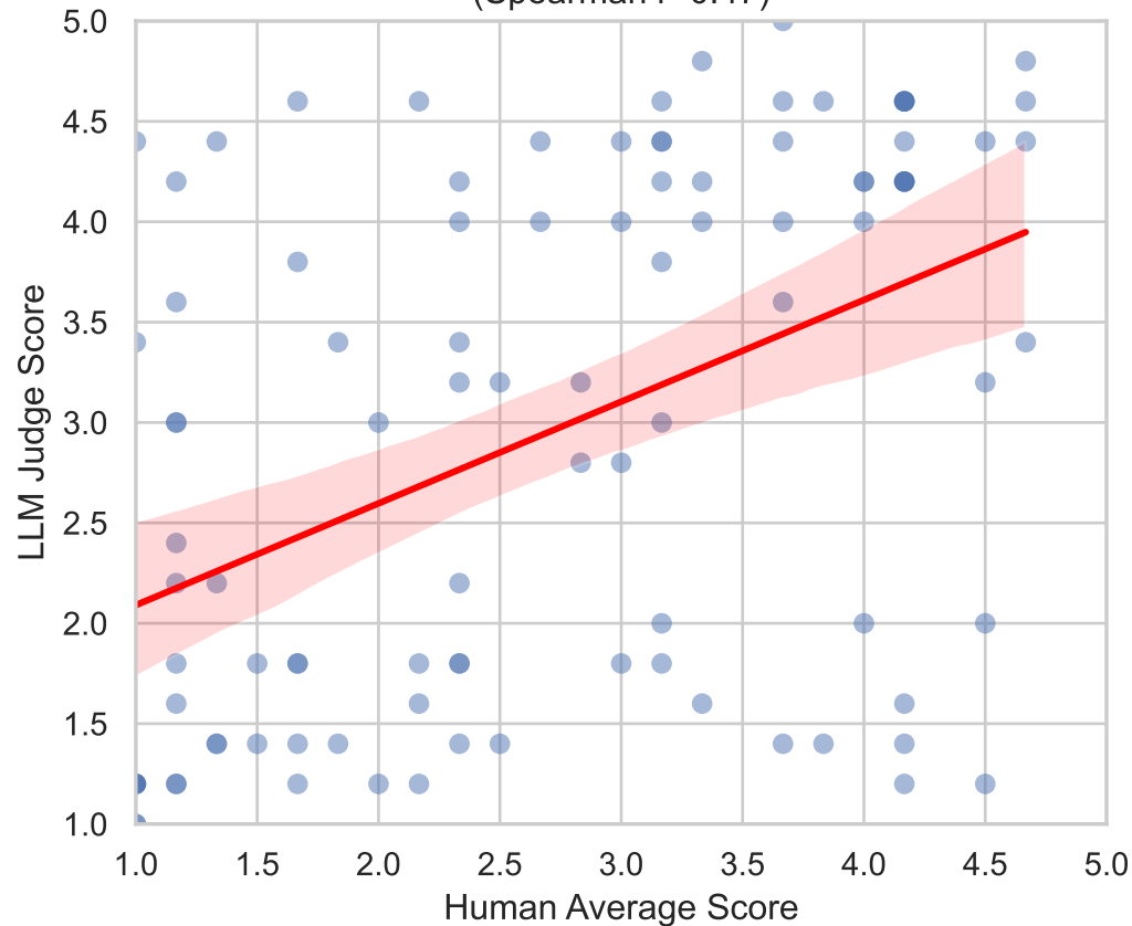
Political: Human vs LLM (Spearman r=0.47 )
