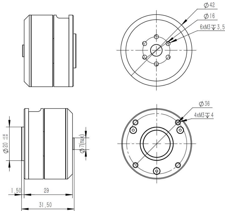
尺寸图 (Dimension)
