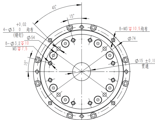
尺寸图 (Dimension)
