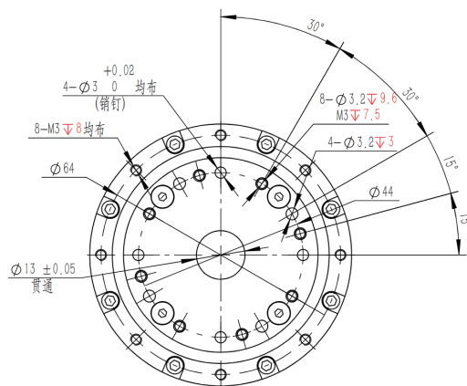
尺寸图 (Dimension)
