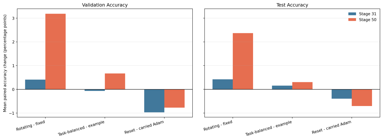
Main effects averaged over the other two paired factors
