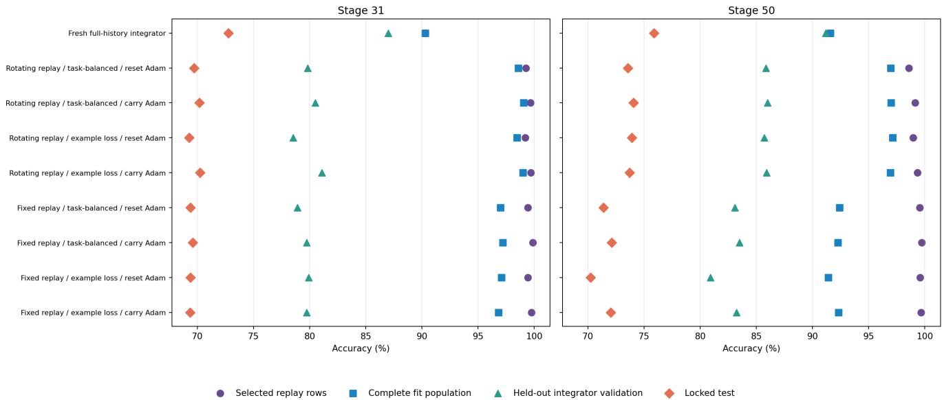
Memorization check: selected rows versus unseen populations
