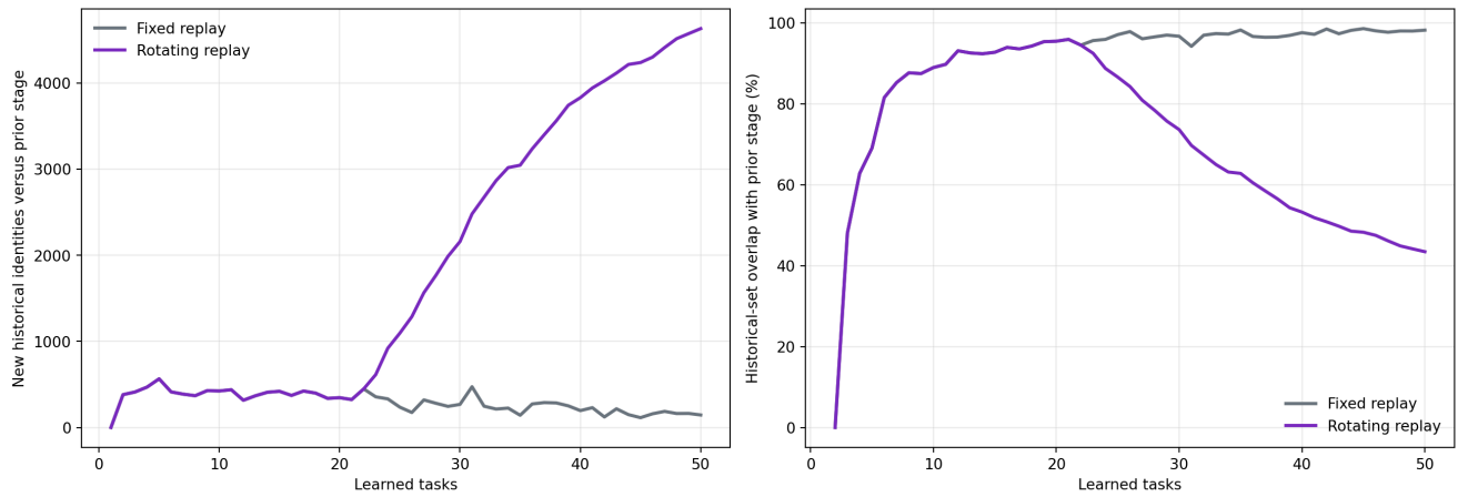
Stage-keyed replay changes which old examples train the integrator
