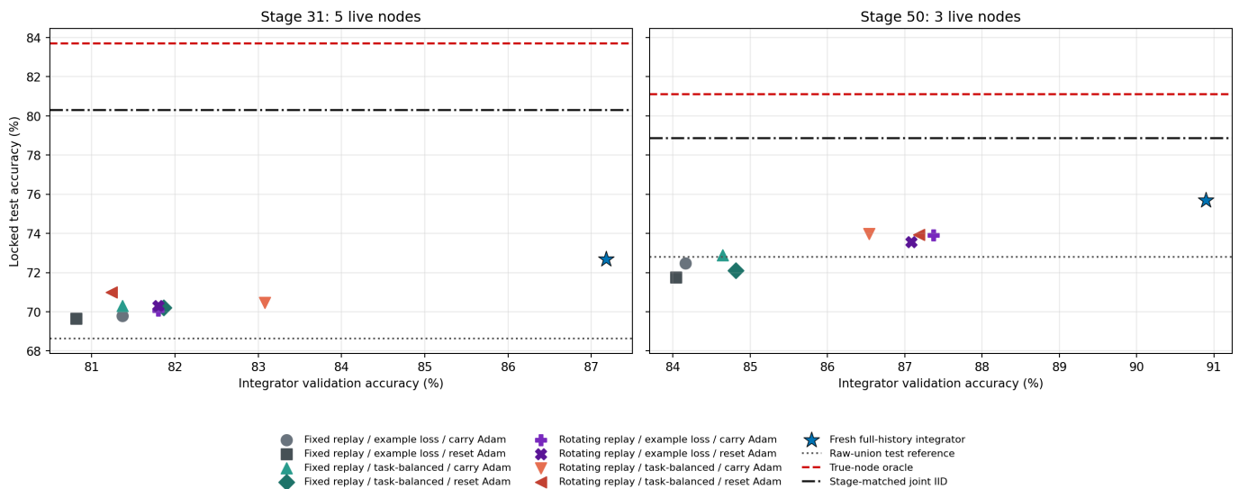
Replay adaptation: validation-selected evidence and locked test accuracy
