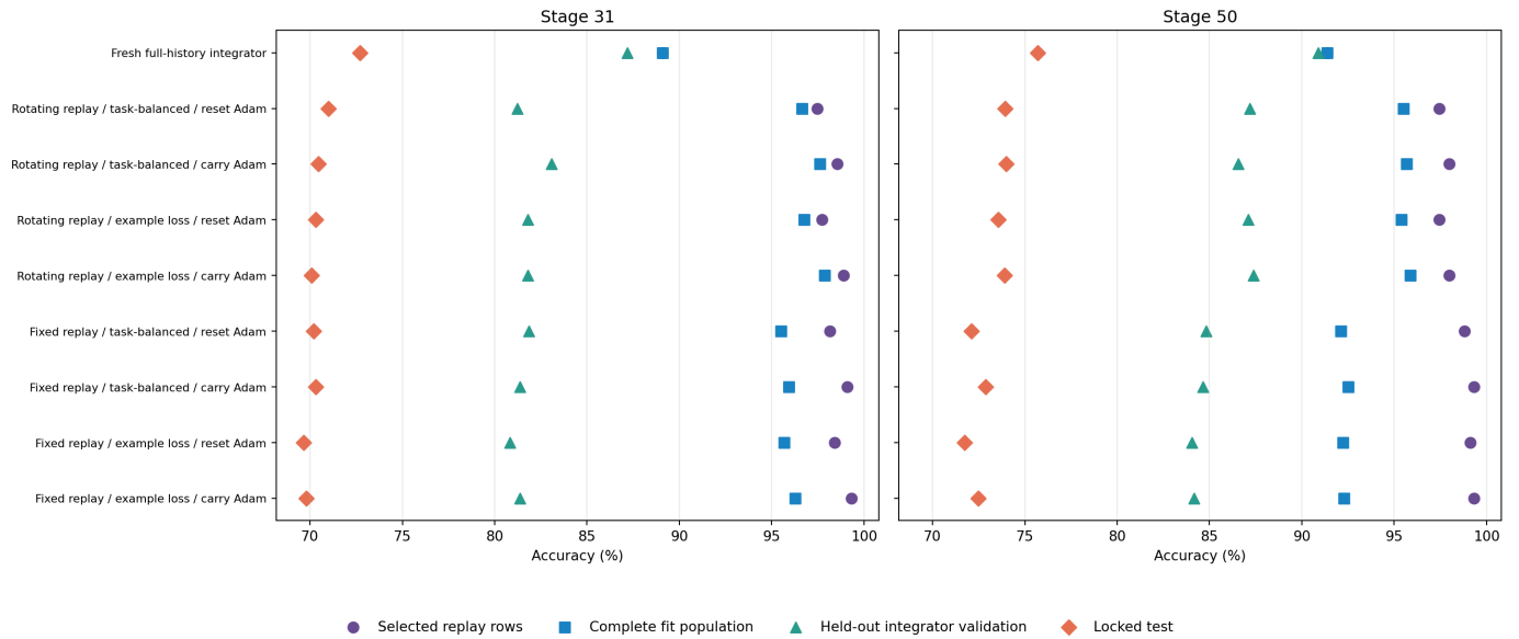
Memorization check: selected rows versus unseen populations
