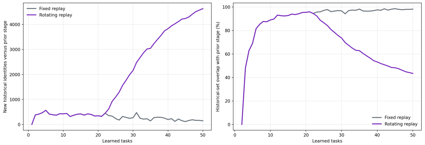
Stage-keyed replay changes which old examples train the integrator
