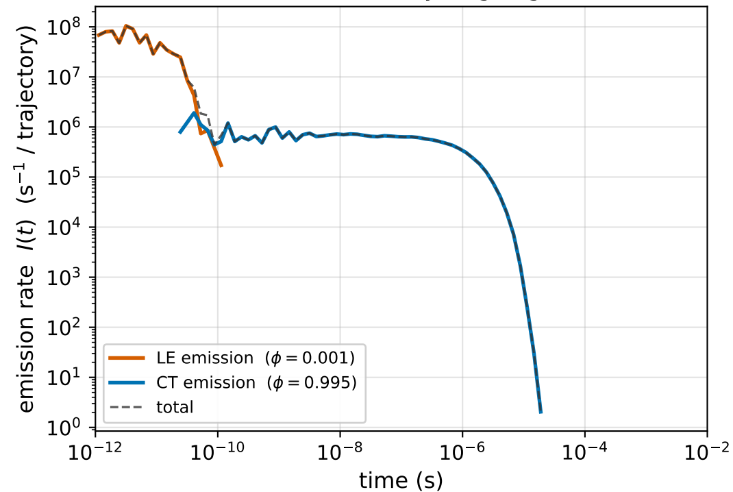
Emission decay (log-log)
