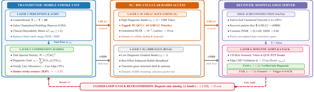
Fig. 4. The Proposed 4-Layer Diagnostic-Aware Tele-Radiology Architecture. Layer 1 embeds the Causal Safety Audit (CSA); Layer 2 optimizes source compression via DARDO; Layer 3 enforces 5G URLLC slicing for critical stroke bands; Layer 4 closes the loop via 128-byte semantic tokens and targeted S-NACK retransmissions.
