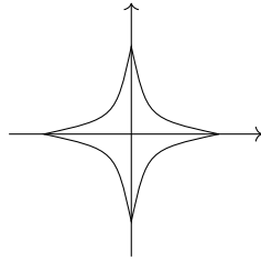
liquid: \{\sum |x_s|^\beta \leq c\}
