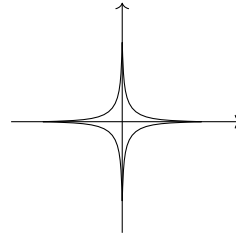
gaseous: \{\sum f_k(x_s) \leq c\}
