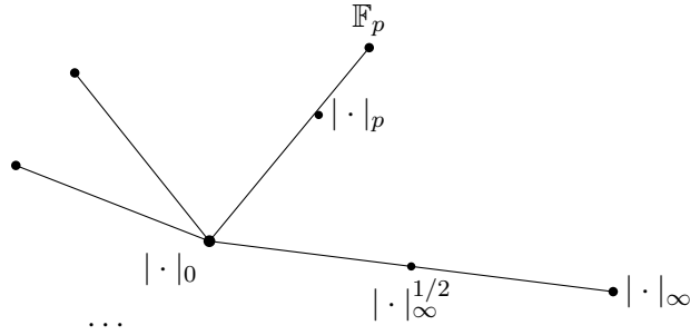
Figure 22.1: The Berkovich tree \mathcal{M}^{\text{Berk}}(\mathbb{Z}) : trivial norm at the centre, one branch per prime ending at \mathbb{F}_p , and an archimedean branch ending at the usual absolute value.
