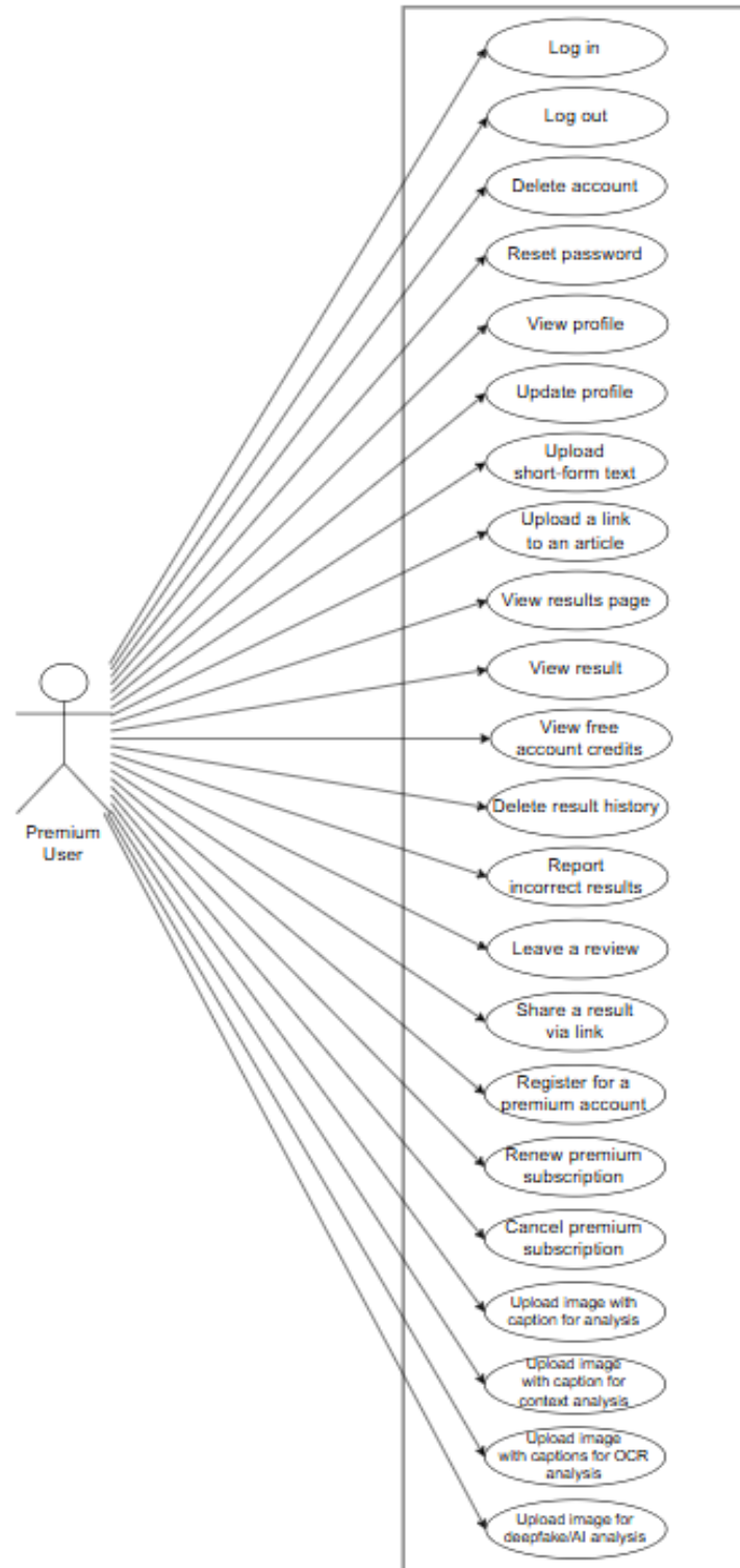
Figure 3.2. Premium User Use Case Diagram
