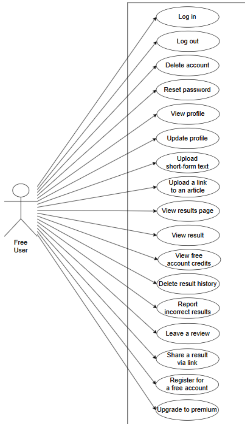
Figure 3.1. Free User Use Case Diagram
