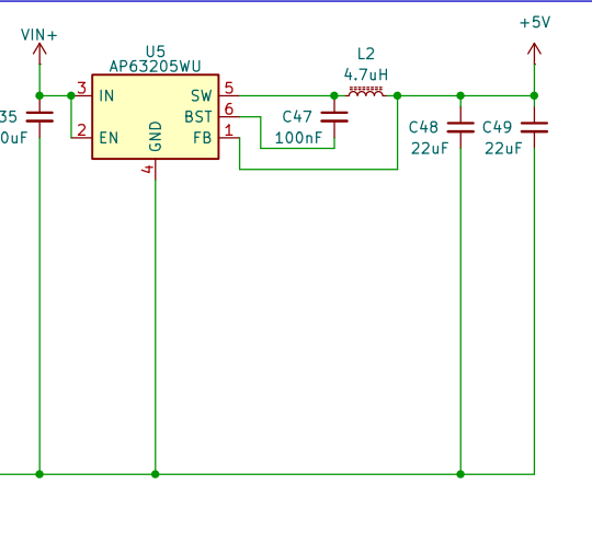
VIN Pin (5.5V - 32V) -> 5V0 Switching Converter
