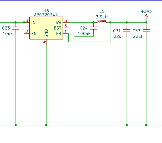
5V -> 3V3 Switching Converter
