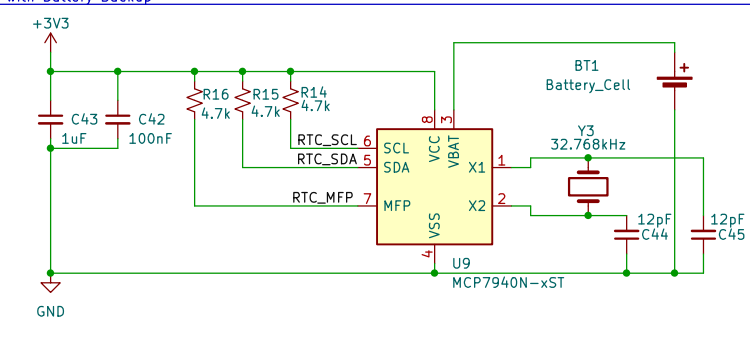
RTC with Battery Backup
