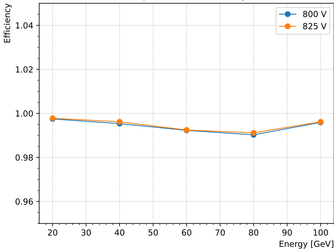
Amplitude-cut efficiency
