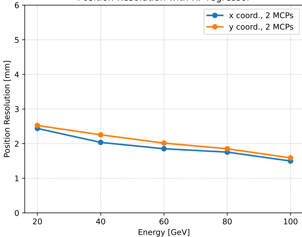
Position Resolution with RF regressor
