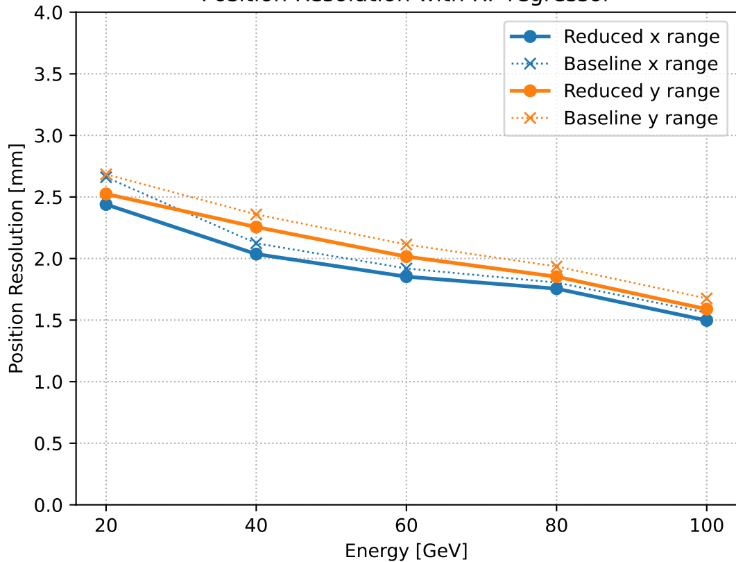
Position Resolution with RF regressor
