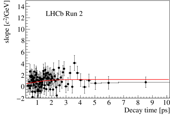
Figure 13: Invariant mass slope as a function of the decay time in the right-hand sideband ( m \in [5.5, 6.2] GeV). Year: 2017s29r2p2; Magnet: Tot; \text{bdtGraNEW} > 0.86 ; Spectrum: PIPI; F. Tagging: None
