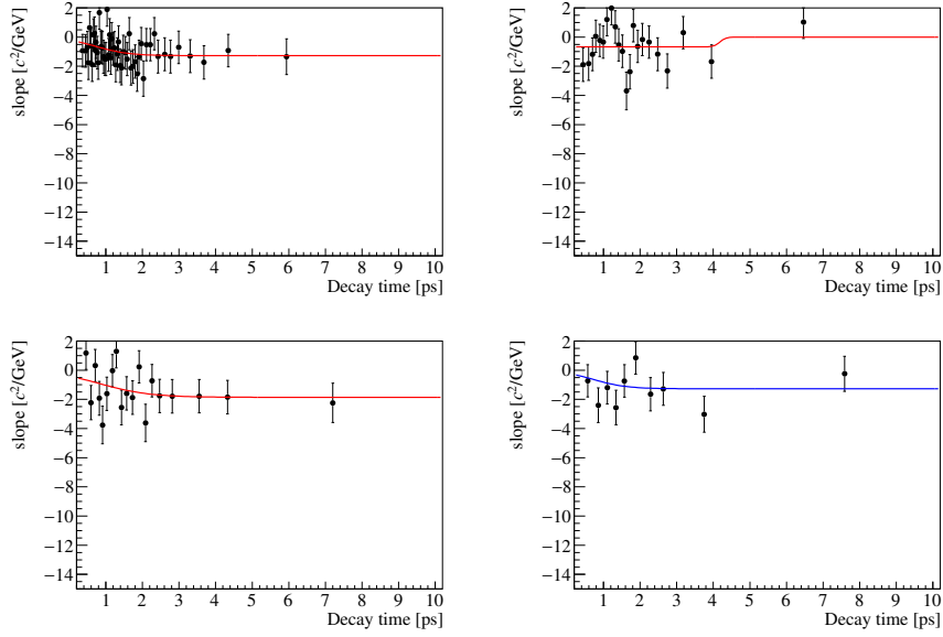
Figure 14: Invariant mass slope as a function of the decay time in the right-hand sideband ( m \in [5.5, 6.2] GeV). Year: 2017s29r2p2; Magnet: Tot; \text{bdtGraNEW} > 0.86 ; Spectrum: PIPI; F. Tagging (from top-left to bottom-right): OS and SS tagged, OS only tagged, SS only tagged, untagged.
