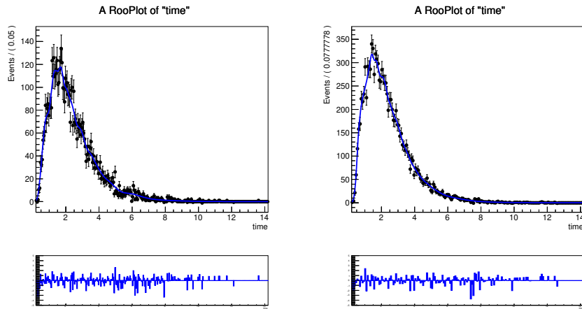
Figure 16: Templates for partially reconstructed background. Left: SS-untagged, right: SS-tagged. Year: 2017s29r2p2; Magnet: Tot; \text{bdtGraNEW} > 0.86 ; Spectrum: PIPI.
