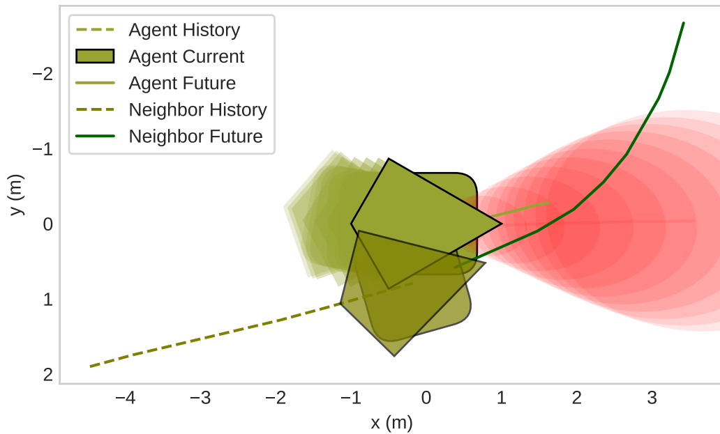
crowds_zara01/t=148 AgentType.PEDESTRIAN/8
