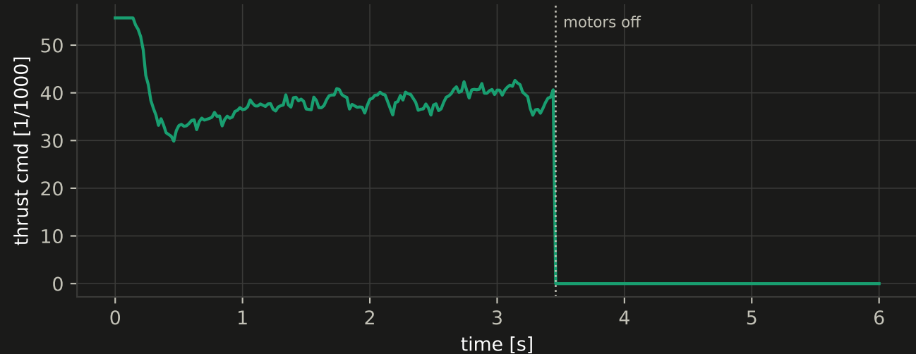
Thrust command (per motor) - geofence
