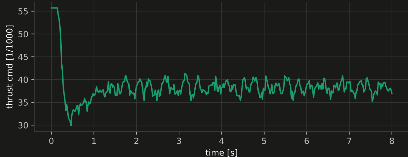
Thrust command (per motor) - hover
