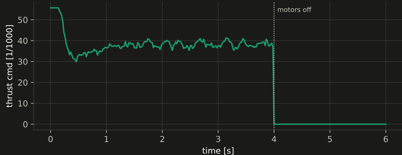
Thrust command (per motor) - kill_switch
