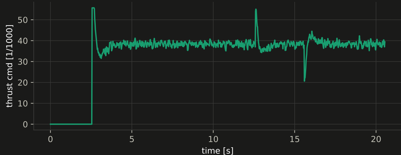
Thrust command (per motor) - ros_steps
