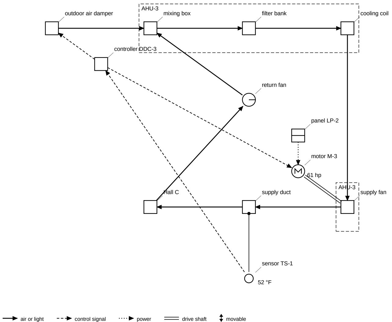
Figure 1. AHU-3 air system schematic
