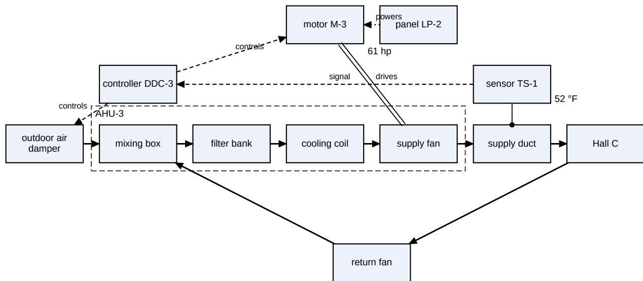
Figure 1. AHU-3 air system schematic
