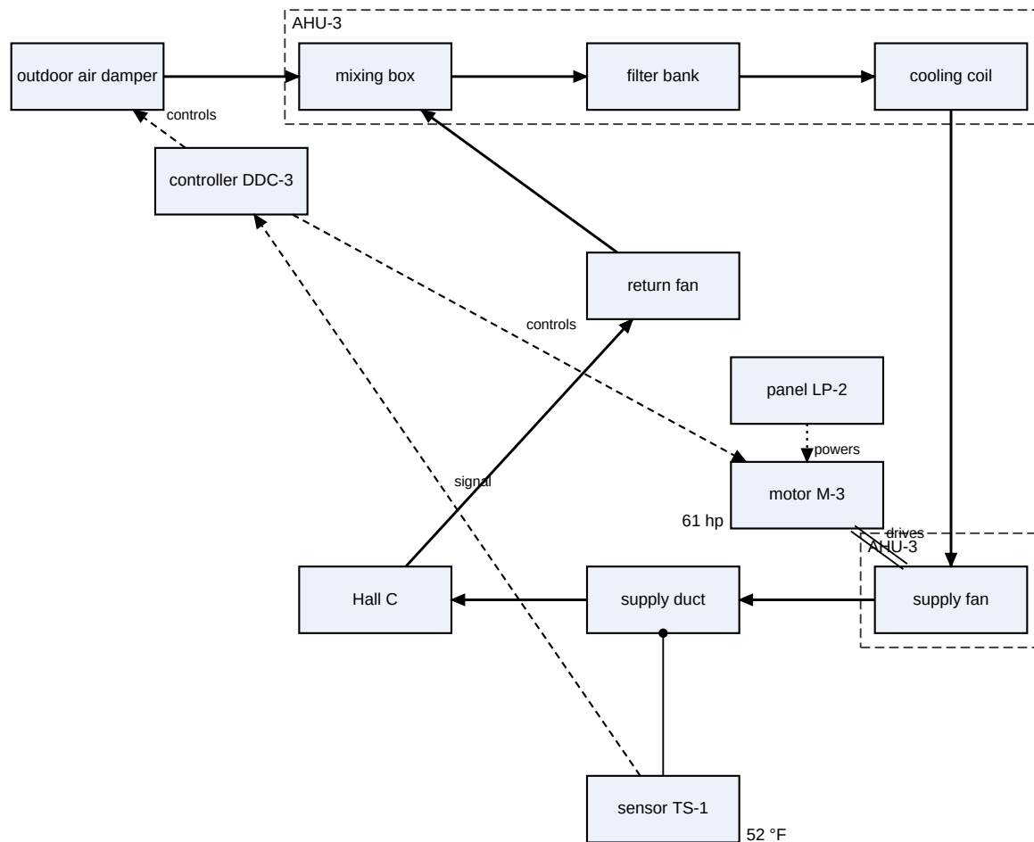
Figure 1. AHU-3 air system schematic
