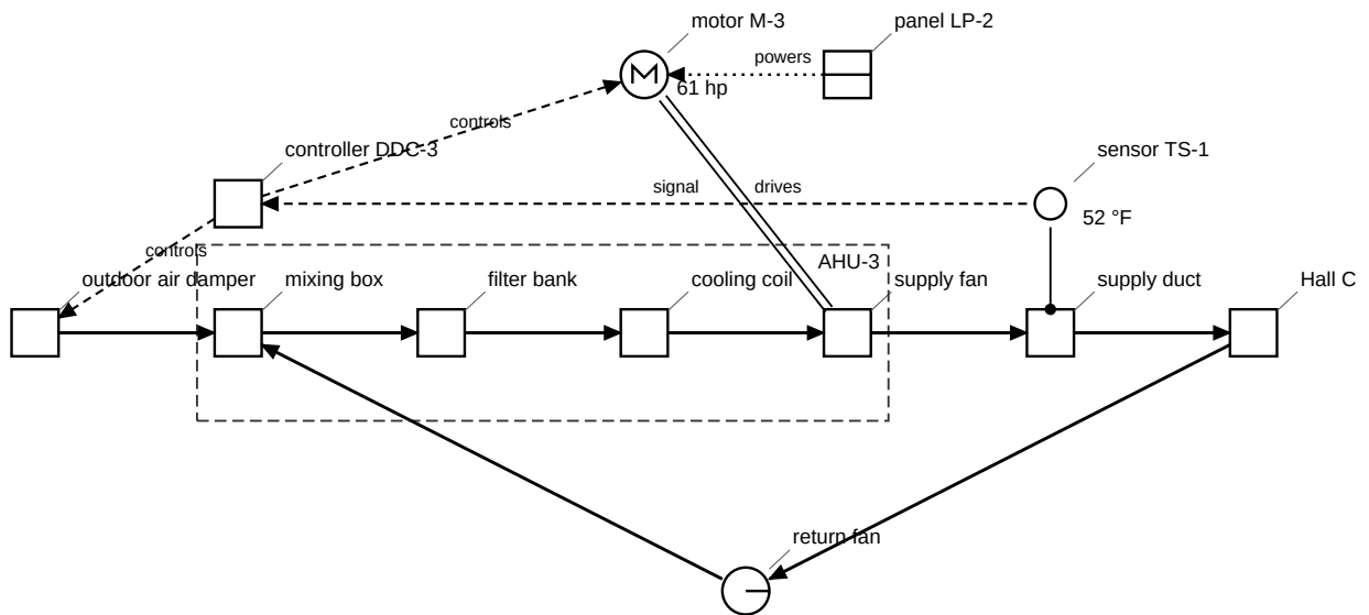
Figure 1. AHU-3 air system schematic
