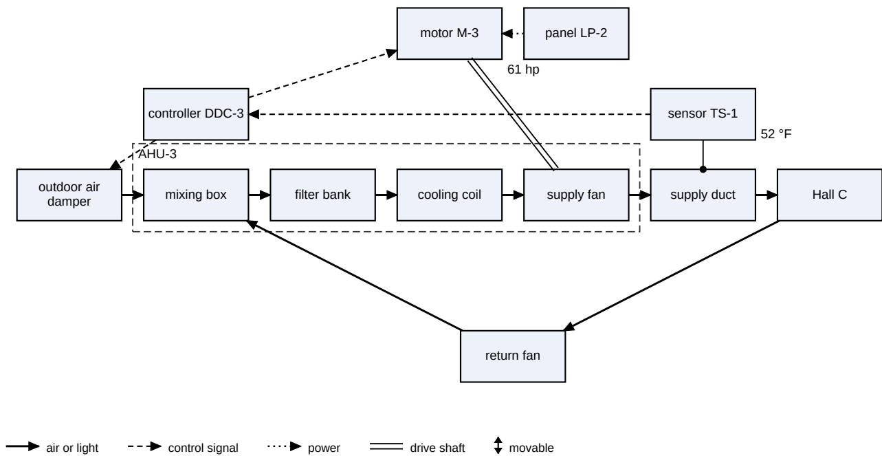
Figure 1. AHU-3 air system schematic
