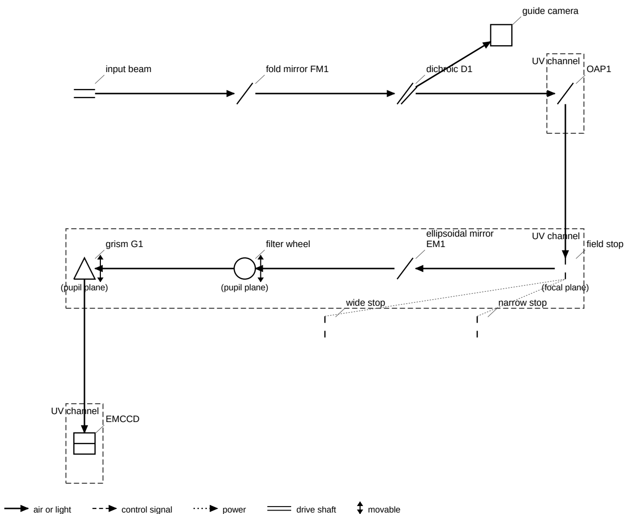
Figure 1. UV channel optical layout
