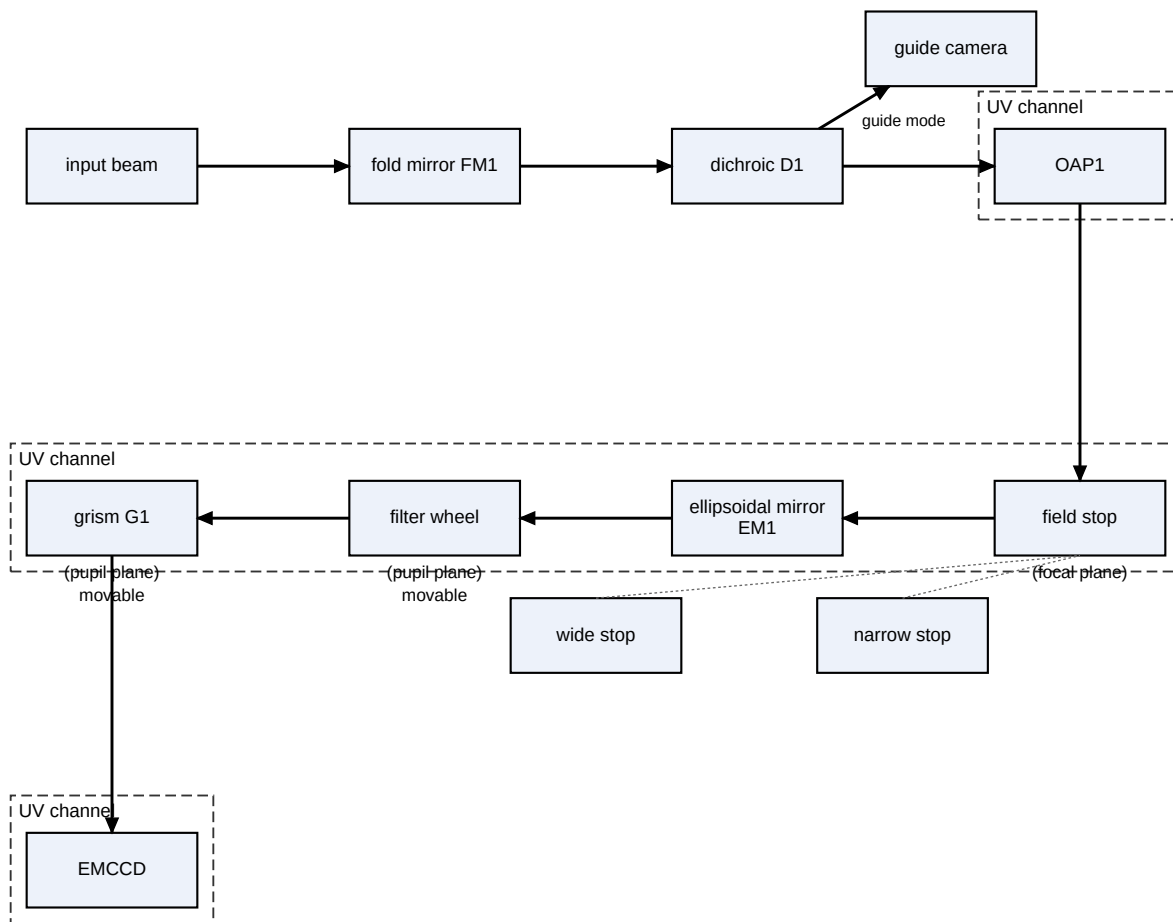
Figure 1. UV channel optical layout
