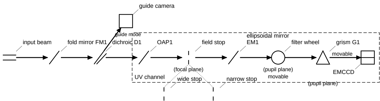
Figure 1. UV channel optical layout
