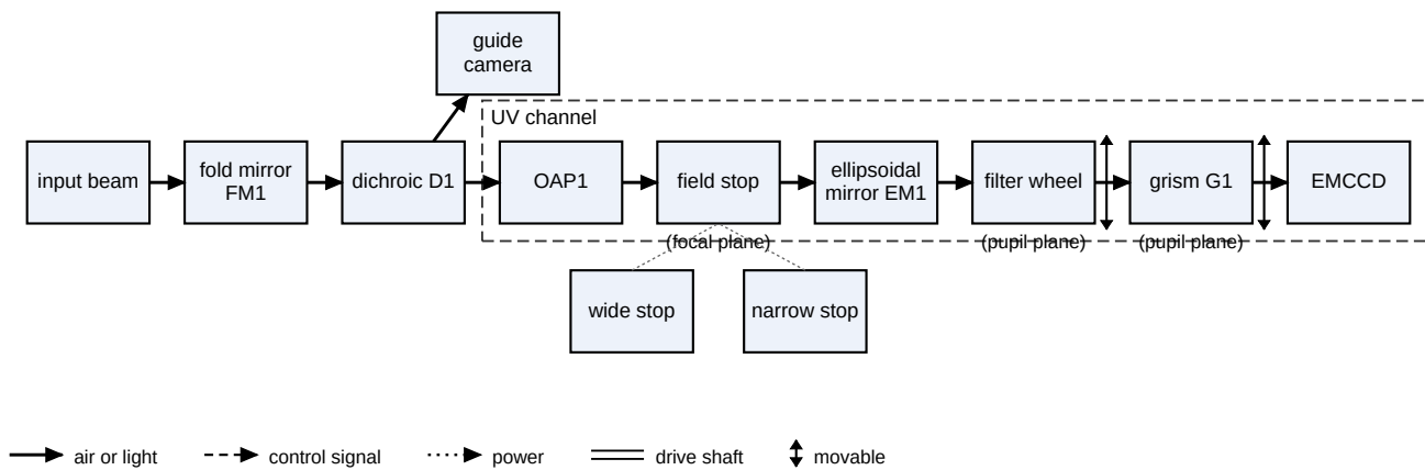
Figure 1. UV channel optical layout
