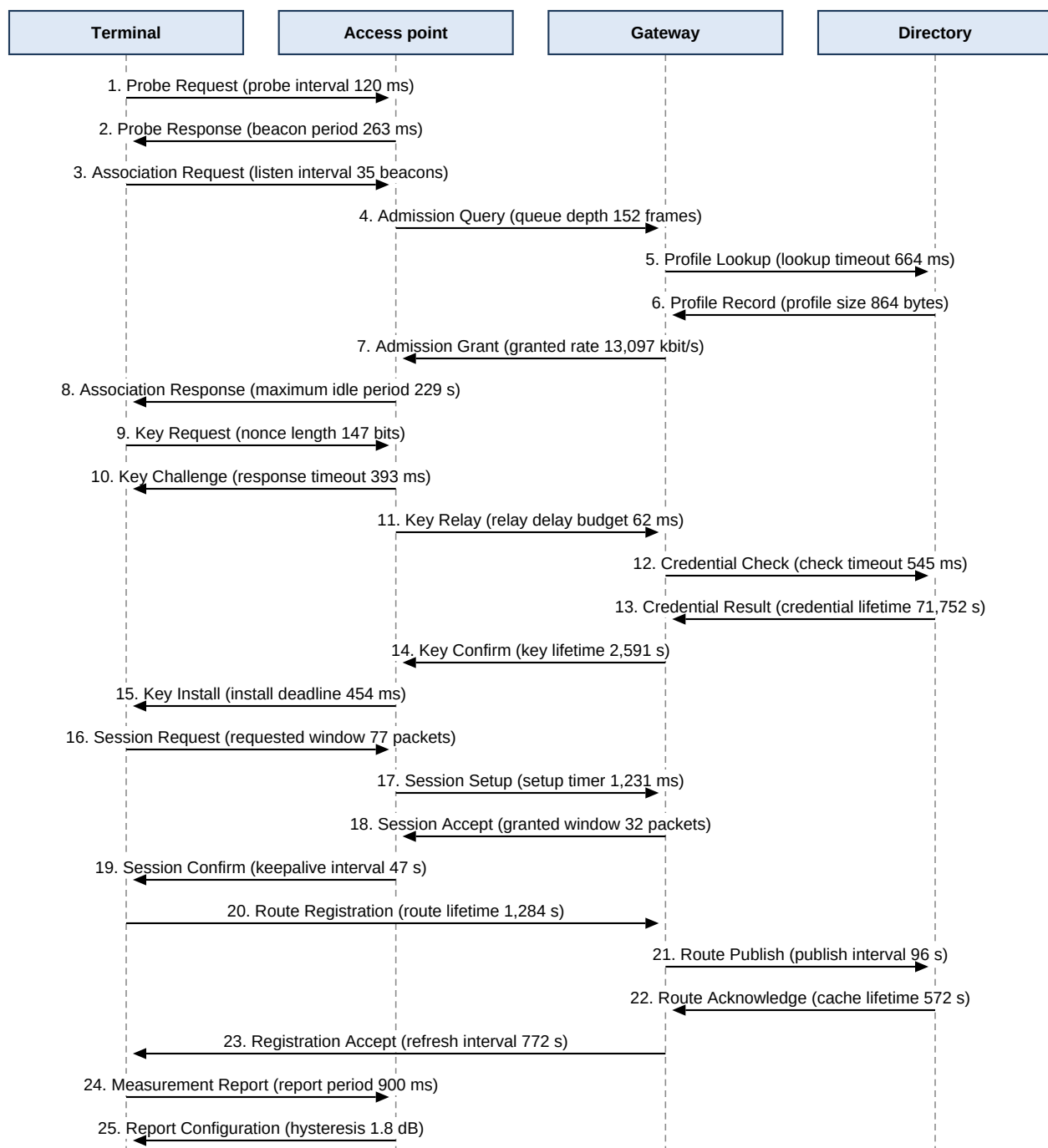
Figure 1. Attach procedure
