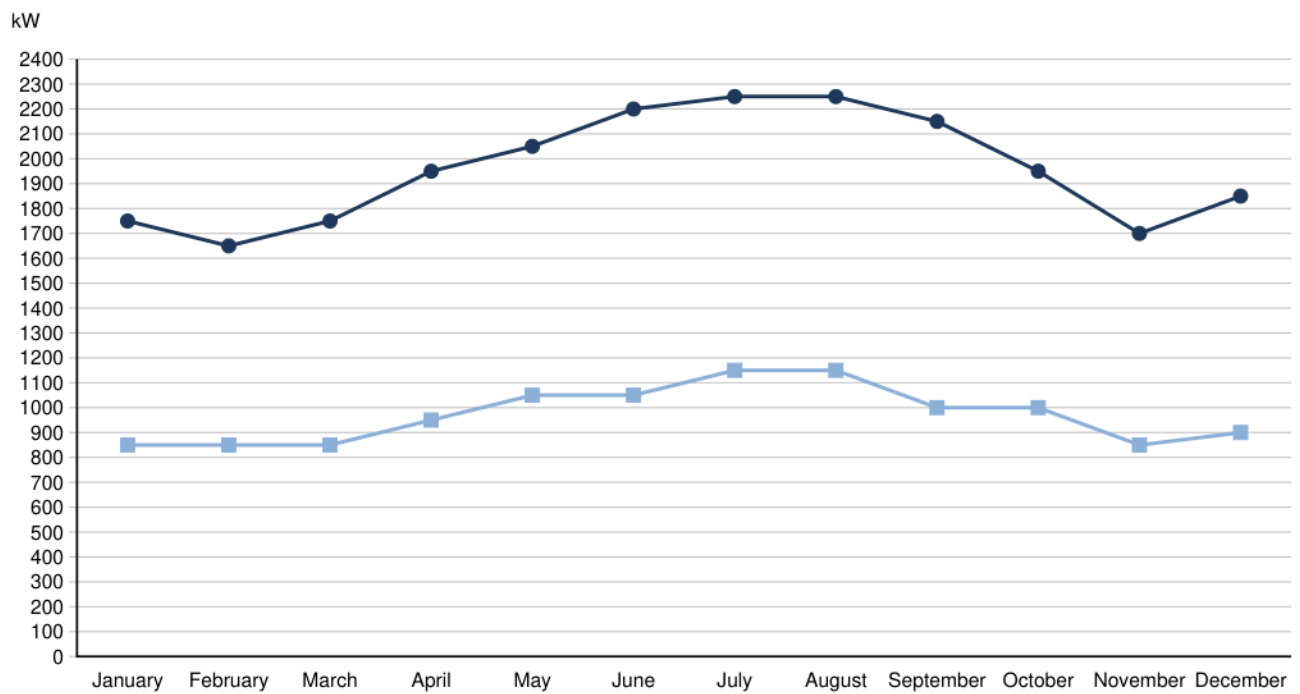
Figure 2. Monthly peak demand by substation (circles: North substation; squares: South substation)
