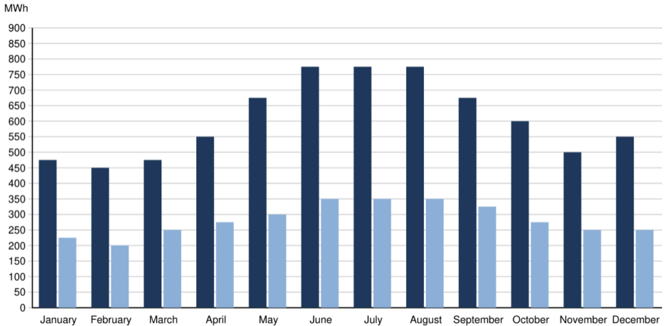
Figure 1. Monthly electricity use by substation (dark bars: North substation; light bars: South substation)
