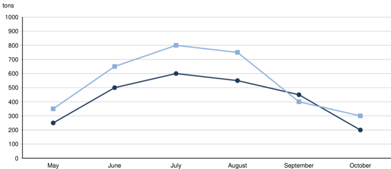
Figure 2. Monthly peak cooling load of the two options (circles: Option 1, chilled beams; squares: Option 2, VAV baseline)
