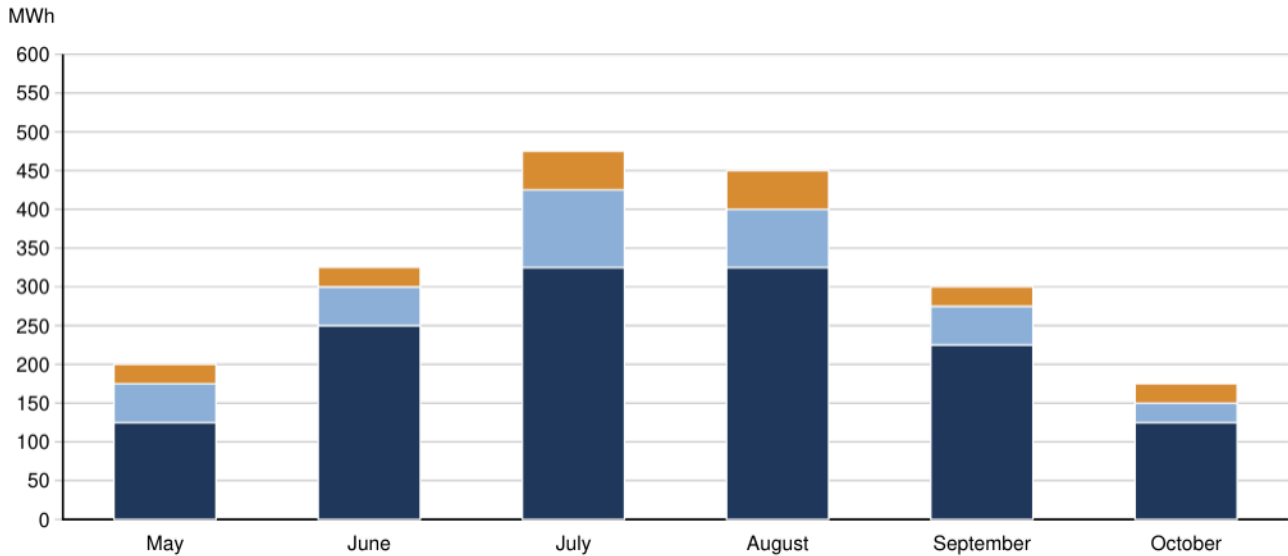
Figure 1. Hall C monthly energy by end use, May to October (dark: cooling; light: fans; orange: lighting)
