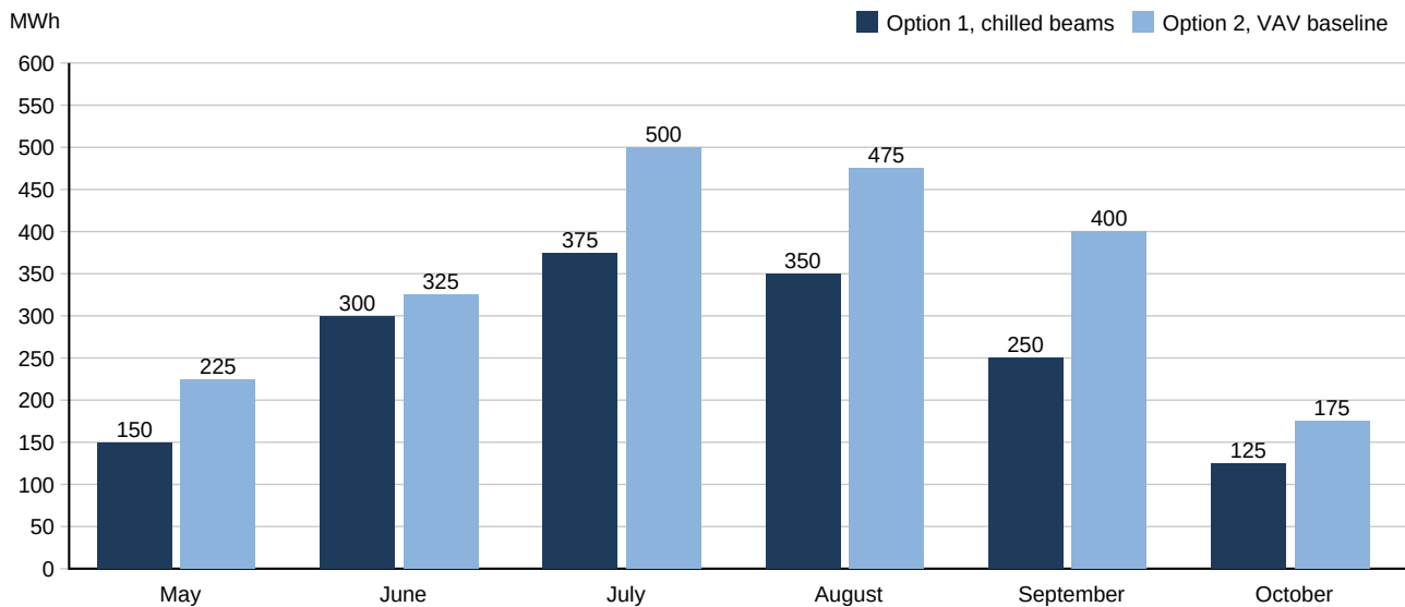
Figure 1. Monthly cooling energy, May to October
