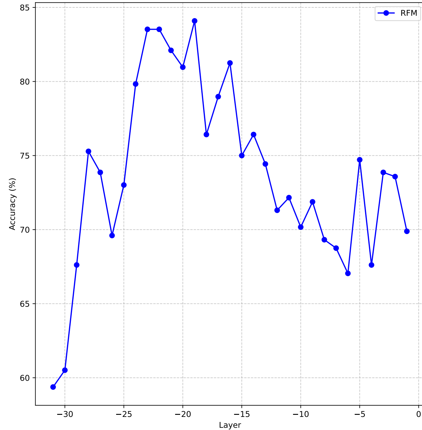
AgentHarm, Average Test Accuracies Across Layers for Llama-3-8b-it
