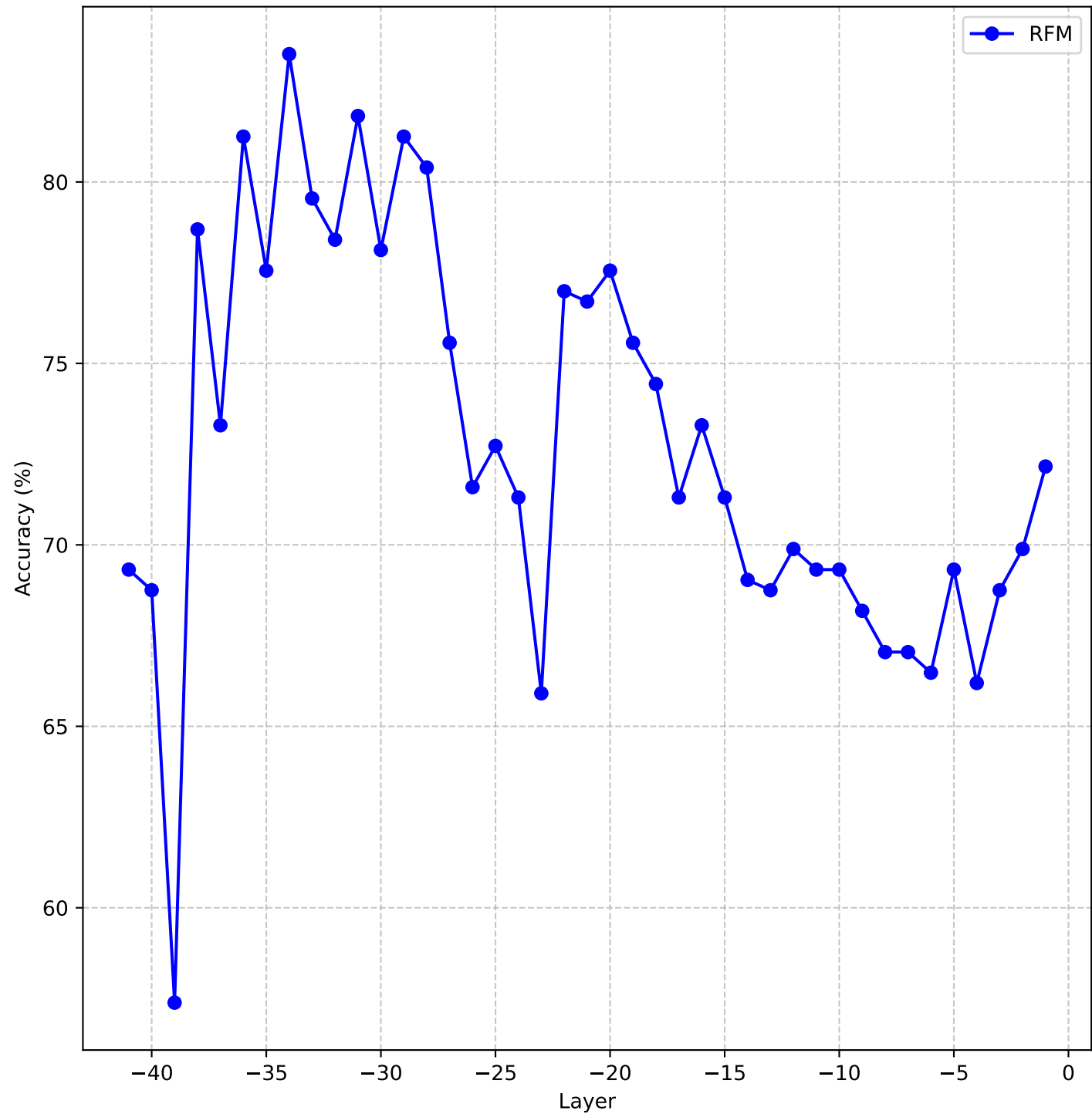
AgentHarm, Average Test Accuracies Across Layers for Gemma-2-9b-it
